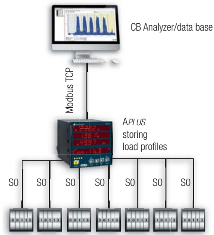
Example of a simple energy management system
